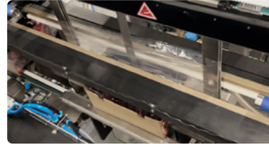
3 Bag stretching & air removal
