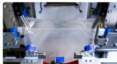
3 Bag spreading
